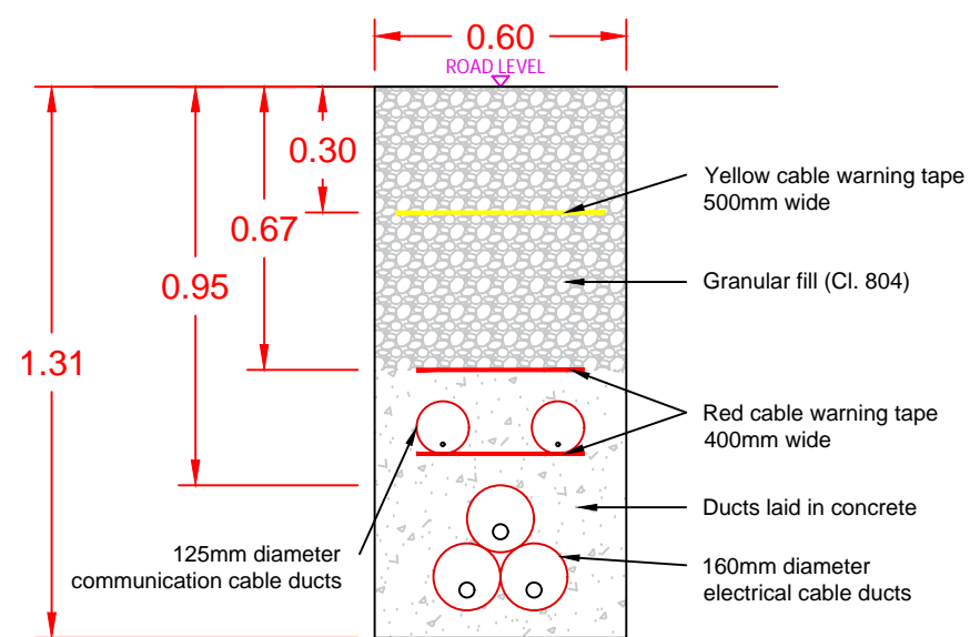
110kV CABLES TRENCH - TYPICAL SINGLE CIRCUIT TRENCH SECTION THROUGH PRIVATE TRACK
