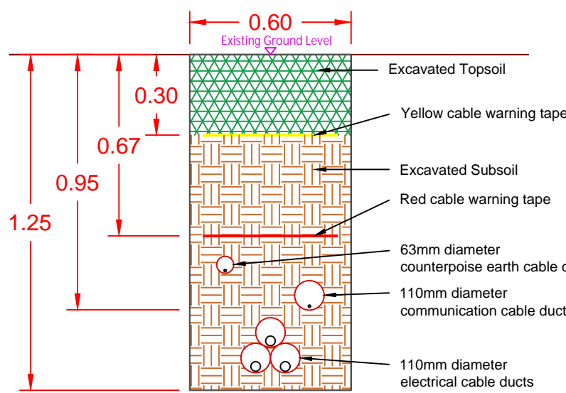
CABLES TRENCH - TYPICAL SINGLE CIRCUIT TRENCH SECTION THROUGH AGRICULTURAL LANDS
